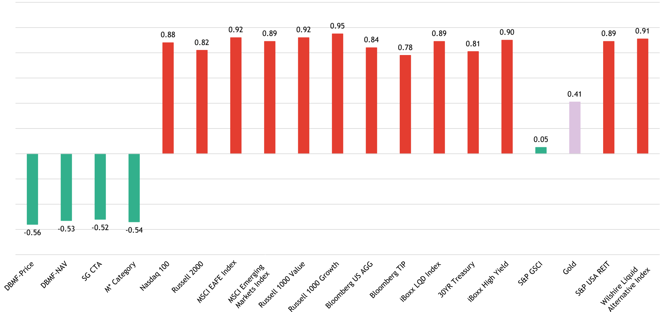
Correlation to S&P500 in 2023
